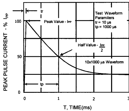
FIG.1 - PULSE WAVE FORM
