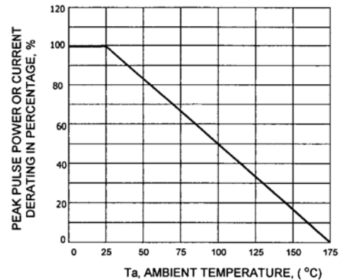
FIG.4 - PULSE DERATING CURVE
